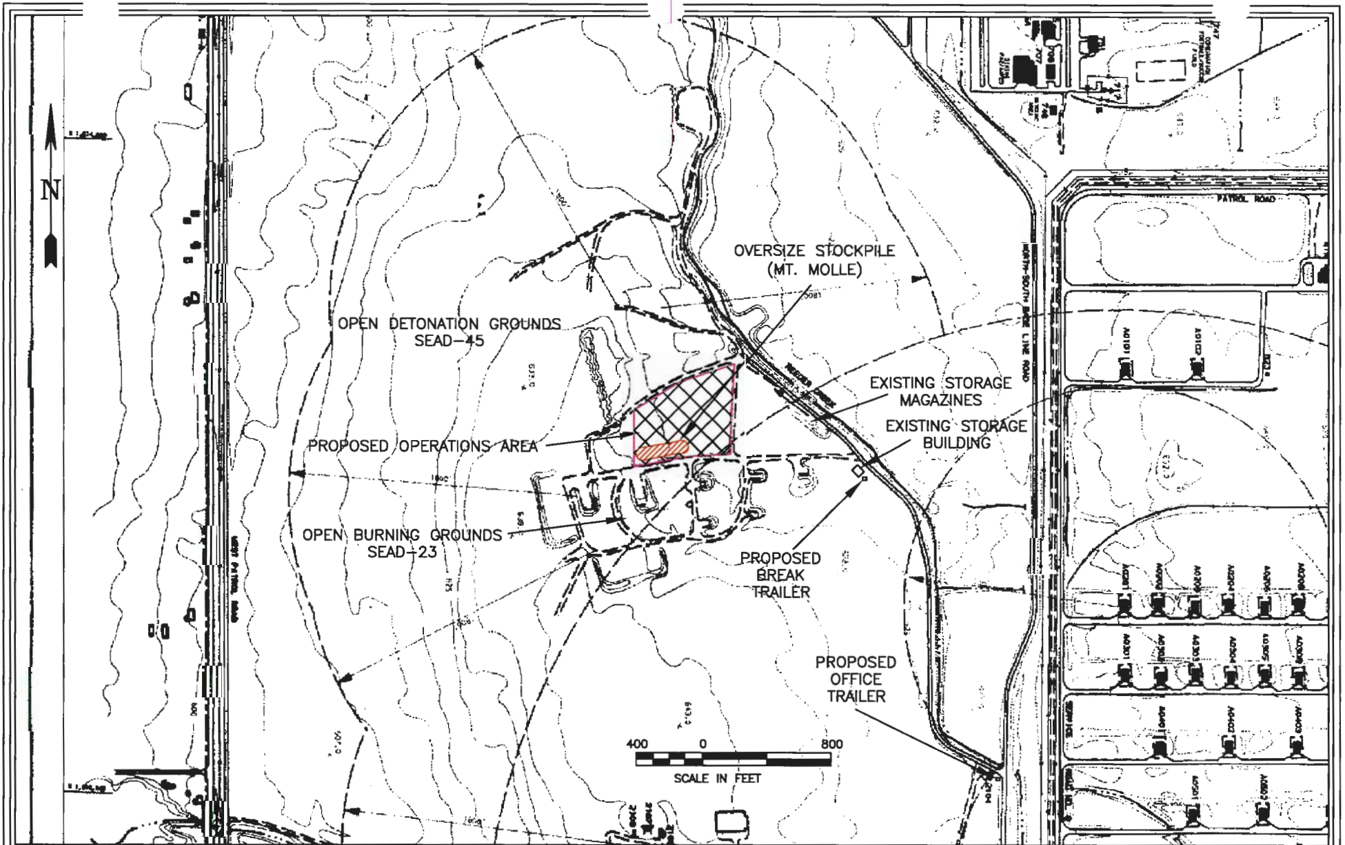
FIGURE 2 - SITE MAP OF OVERSIZE STOCKPILE (MT. MOLLE)
