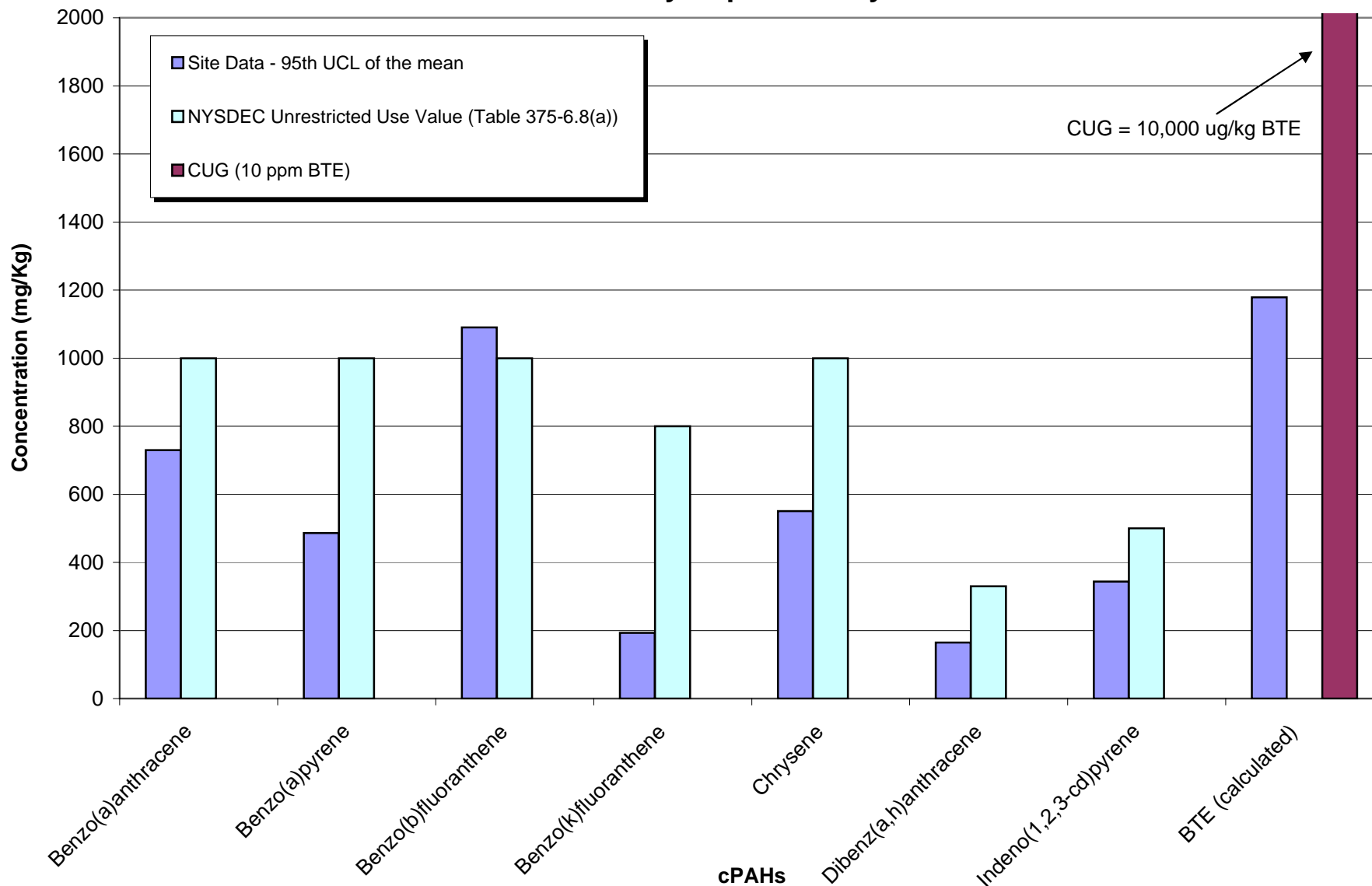
Figure 3-2B Detected cPAH Concentrations in Confirmatory Samples Compared to Benchmark Values SEAD-11 Construction Completion Report Seneca Army Depot Activity
