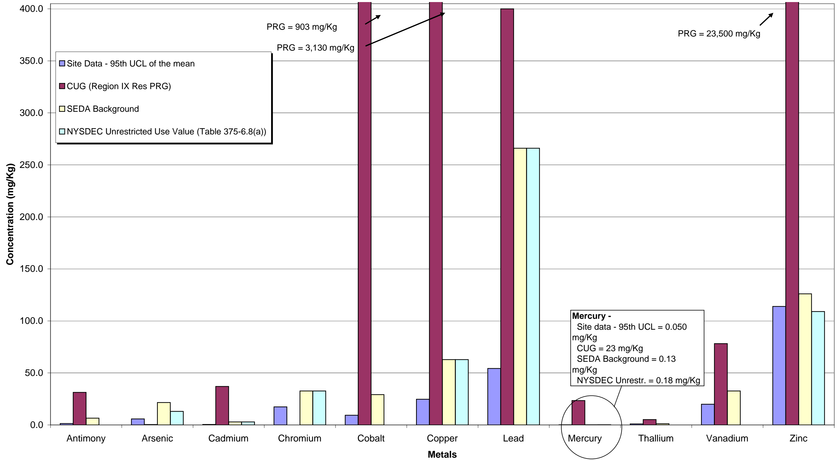
Figure 3-2D Metals Concentrations in Confirmatory Samples Compared to Benchmark Values SEAD-11 Construction Completion Report Seneca Army Depot Activity
