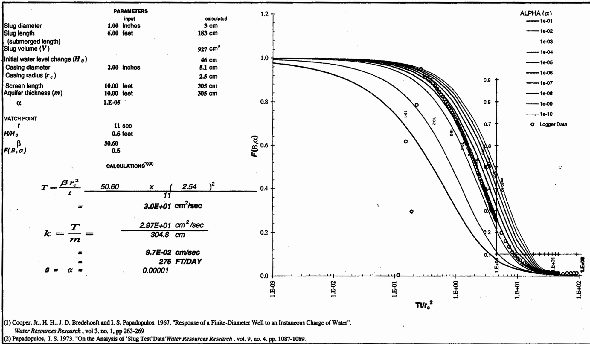
FIGURE 1.1 CONFINED AQUIFER SLUG TEST MONITORING WELL MW-1 WITHDRAWAL TEST
