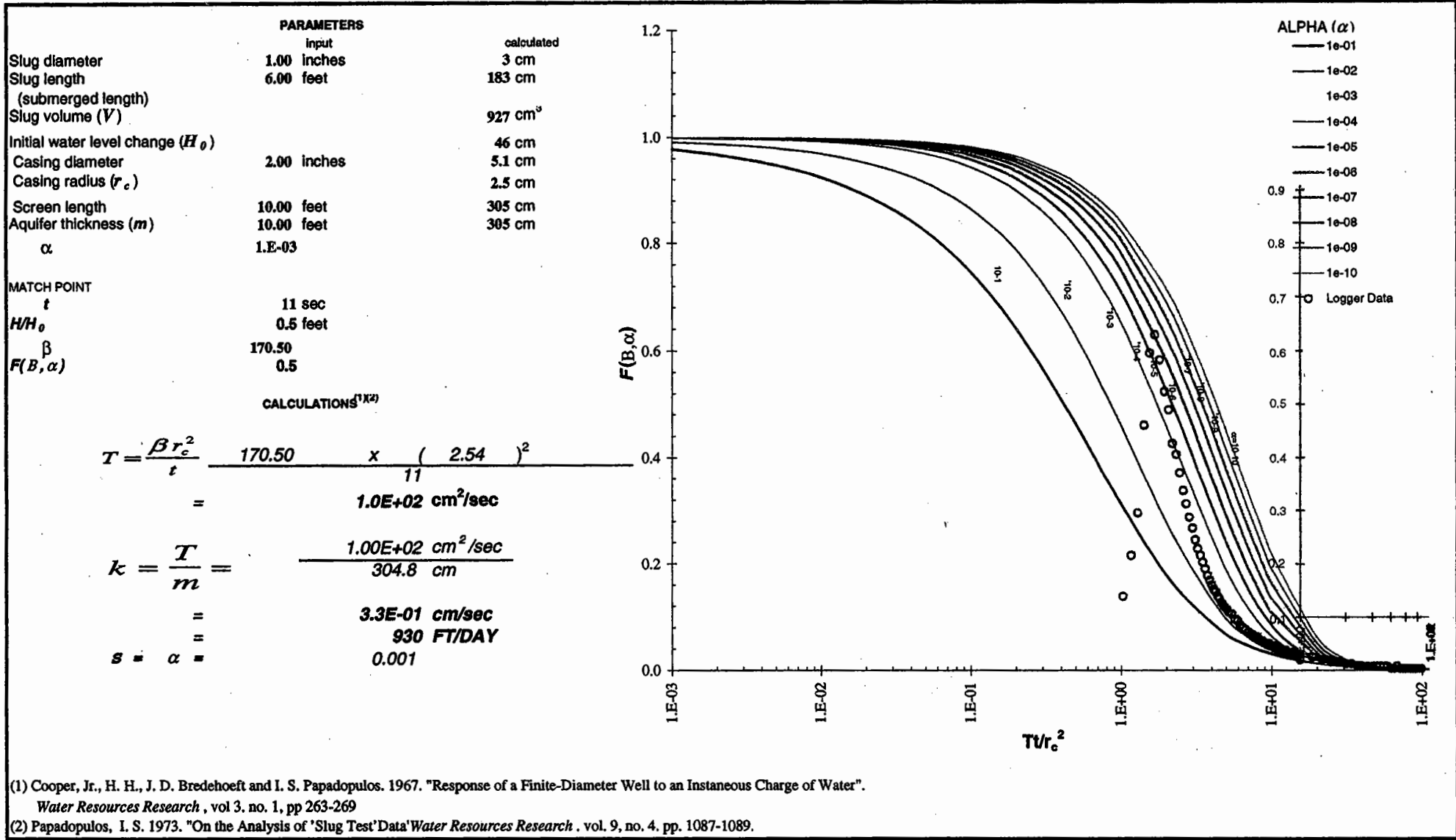
FIGURE 1.5 CONFINED AQUIFER SLUG TEST MONITORING WELL MW-3 WITHDRAWAL TEST
