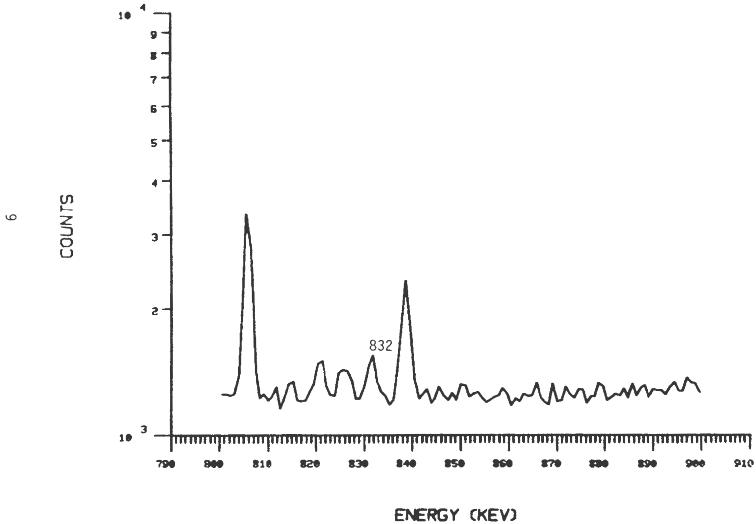
Figure 2. Soil Spectrum Middle Energy
